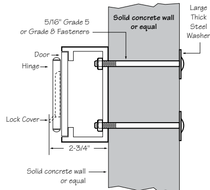
Series 1650 Hinged Door Surface Mounted
